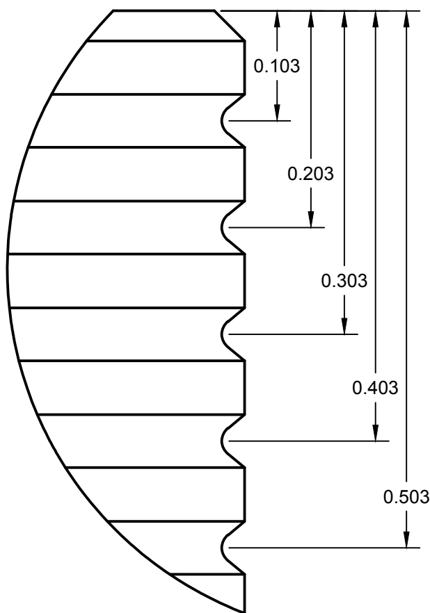
DETAIL A SCALE 8:1
