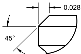
DETAIL D SCALE 8:1
