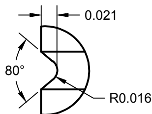
DETAIL C SCALE 8:1
